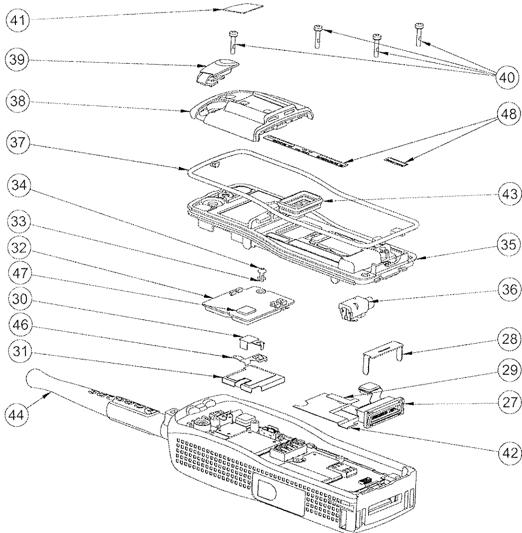
Figure 24 MTP850 — Exploded View 3
